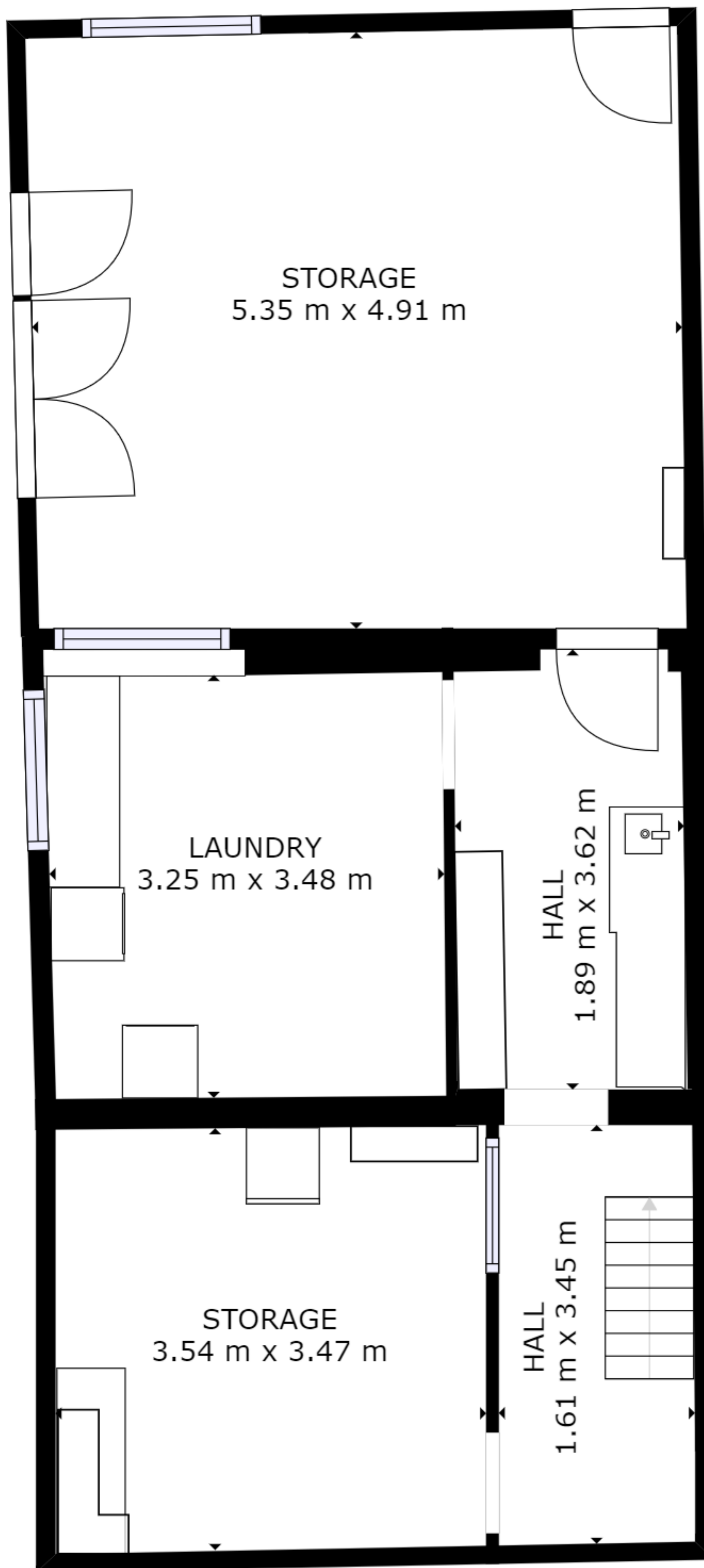
FLOOR 1
