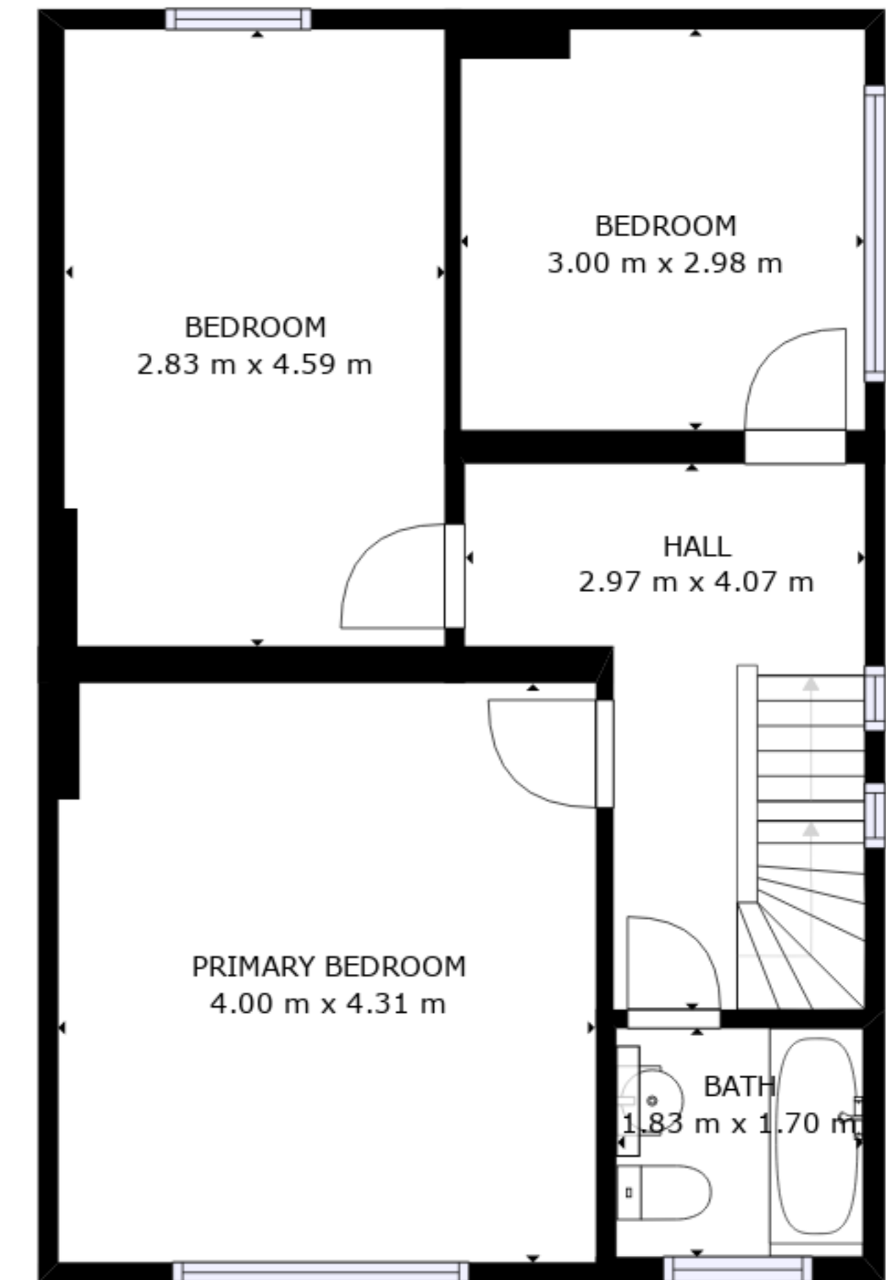
FLOOR 3
