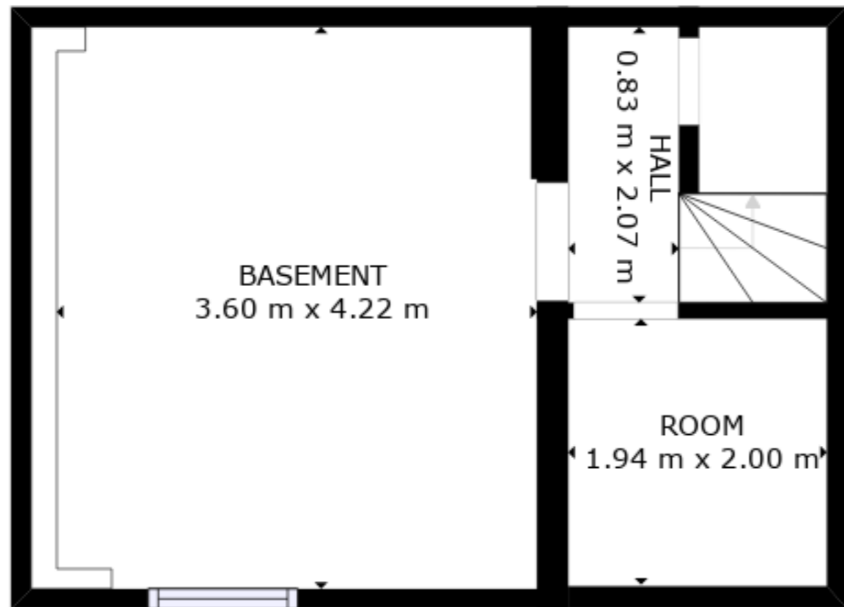
FLOOR 1
